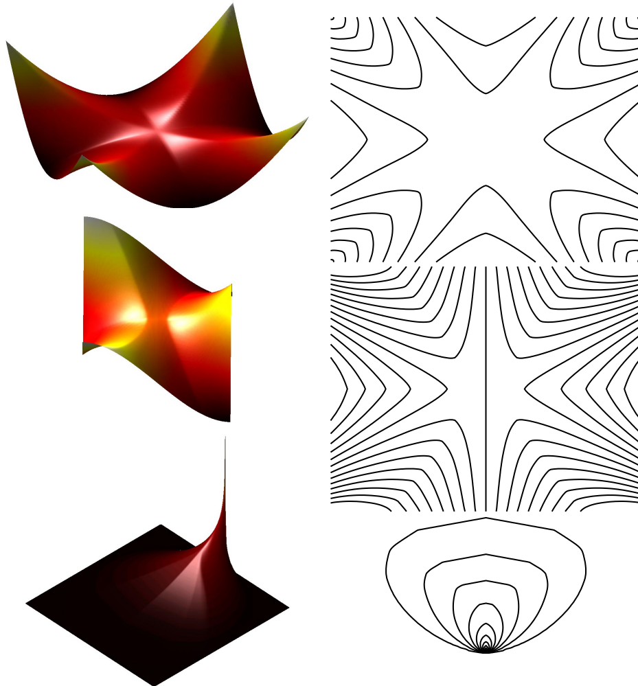
FIGURE 2. Surface and contour plots using the 25 neighbor method, for boundary data |x| , and x^3 - 3xy^2 , on a square, and boundary data the characteristic function of a point, on a circle.
