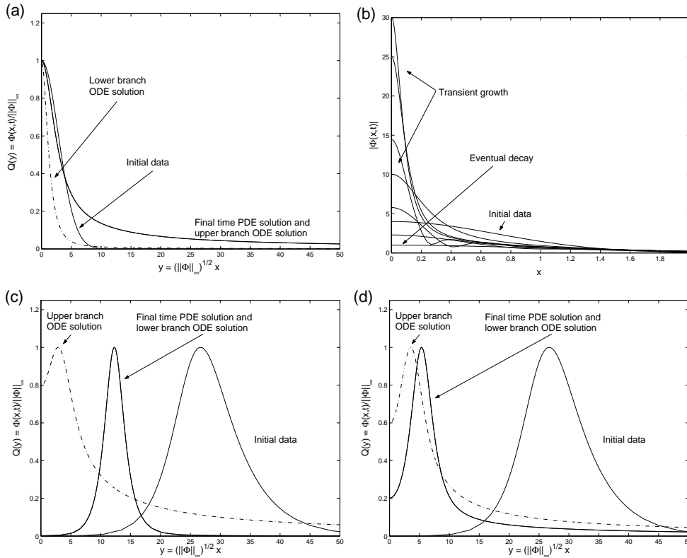
FIG. 7.2. Numerical simulations of the full CGL for monotone and non-monotone initial conditions. The initial solution, t = t_0 , and some intermediate time-steps, where t_i < t_{i+1} , are given, as well as the final-time profile at T^- . Furthermore, the ODE solutions that were observed for the same \varepsilon on both the upper and the lower part of the k = 1 , resp k = 2 , solution branch are given. In all but one case, the profiles are presented in rescaled coordinates. (a) Monotone initial data where \varepsilon = 0.1 < \varepsilon_1^* < \varepsilon_2^* converge to a monotone final profile found on the upper part of the k = 1 solution branch. (b) Monotone initial data, plotted in the physical coordinates, decay to the zero solution for \varepsilon_1^* < \varepsilon = 0.22 < \varepsilon_2^* . (c) Non-monotone initial data, where \varepsilon = 0.1 < \varepsilon_1^* < \varepsilon_2^* , converge to a non-monotone final time profile found on the lower part of the k = 2 branch. (d) Non-monotone initial data, where \varepsilon_1^* < \varepsilon = 0.22 < \varepsilon_2^* , also converge to a non-monotone final time profile found on the lower part of the k = 2 branch.
