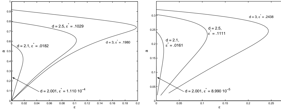
FIG. 3.1. (left) The k = 1 solution branch, the monotone solution is found here, in the (\varepsilon, a) -plane for different choices of d where \delta = 0 . (right) The k = 2 solution branch, the solution Q_2 with two maxima on the real line is found here, in the (\varepsilon, a) -plane for different choices of d where \delta = 0 . The value of the fold bifurcation point \varepsilon_k^*(d) is also given for the branches.
