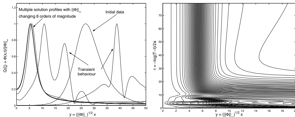
FIG. 7.1. (left) Convergence of a non-monotone initial condition to a multi-bump similarity solution in the rescaled dynamical coordinates. (right) The grid lines of the moving mesh method plotted in the rescaled dynamical coordinates. After an initial transient phase, they are essentially constant in the region of the peak.
