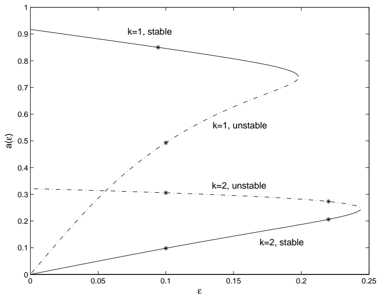
FIG. 1.1. The k = 1 solution branch, the solutions with one maximum on (-\infty, \infty) , and the k = 2 solution branch, the solutions with two maxima on (-\infty, \infty) , plotted in the (\varepsilon, a) -plane where d = 3 and \delta = 0 . The solutions corresponding to the * 's are given in Figure 1.2. On the upper part of the k = 1 solution branch and the lower part of the k = 2 solution branch the solutions are found to be stable whereas on the other parts the solutions are unstable.
