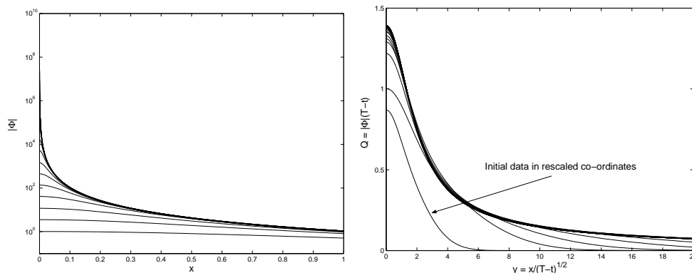
FIG. 2.1. Numerical simulation of the full CGL for d = 3 and \varepsilon = 0.1 . (left) Blow-up in physical coordinates. (right) Blow-up in rescaled coordinates, notice the convergence to a stationary profile.
