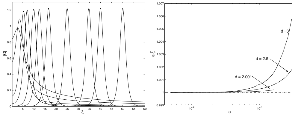
FIG. 3.2. (left) The amplitude of the solutions |Q_2(\xi)| for \xi > 0 as a and \varepsilon are moving along the k = 2 solution branch for d = 3 . The peak of the solution moves to the right as a is decreased to zero. For smaller values of a , the solutions have a similar form and the peak \xi^* is located close to \frac{1}{a} . (Right) The location of the maximum \xi^* along the k = 2 solution branch for various choices of d where a\xi^* is plotted as a function of a .
