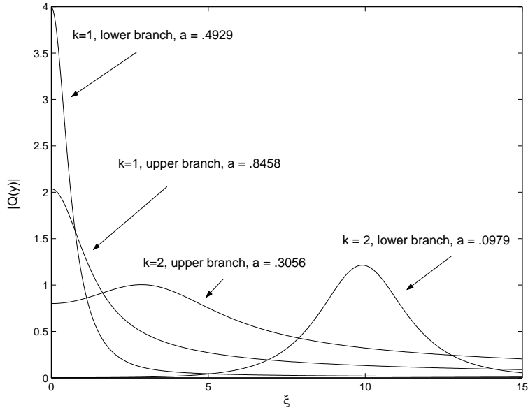
FIG. 1.2. Final-time profiles in the rescaled variables for d = 3 , \delta = 0 and \varepsilon = 0.1 . The solutions correspond to the * 's in Figure 1.1
