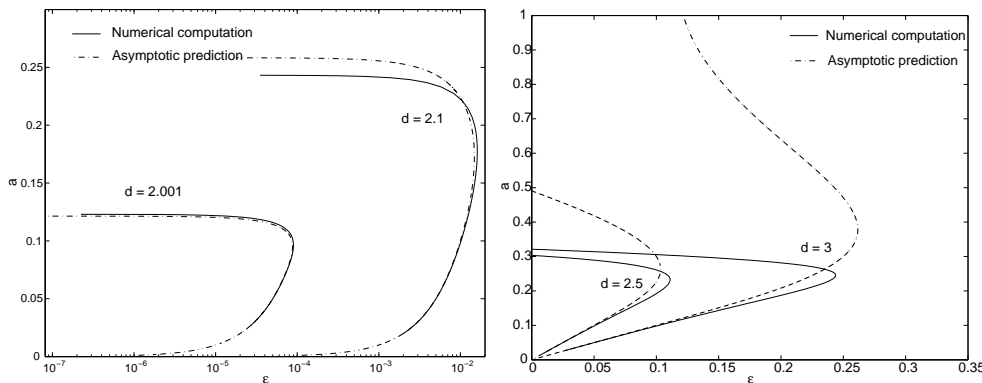
FIG. 3.3. Comparison of the numerical results (solid line) and the asymptotic expansion for a_- and a_+ (dashed line) of the k = 2 solution branch. (left) Here d = 2.1, 2.001 and \varepsilon is plotted on a log-scale. (right) For d = 2.5 and d = 3 .
