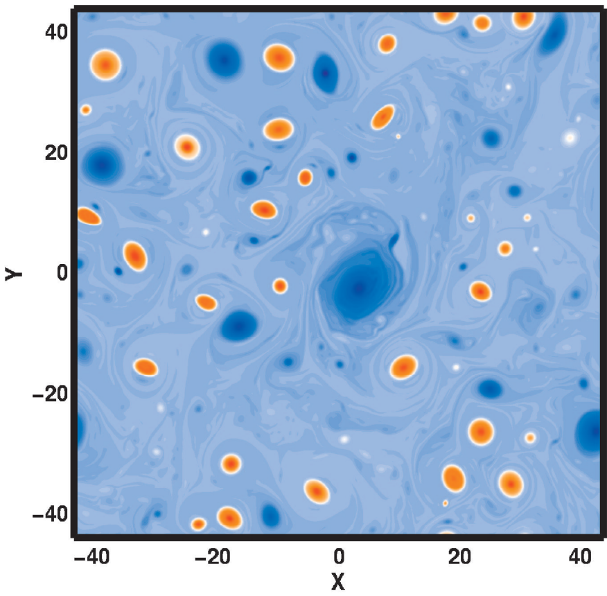
sQG + Theta (t=1000)
