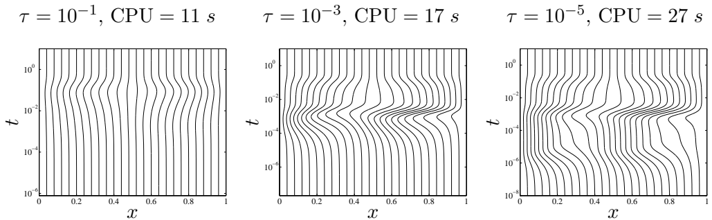
Fig. 3. Mesh trajectories for the given solution (9) (Example 2) using MMPDE6 and the arclength monitor function.
