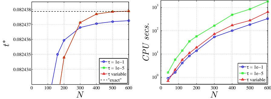
Fig. 8. Left: Comparison of blow-up time estimates for various choices of \tau in the case p = 2 . The best estimate of the exact value of t^* \approx 0.08243786 is shown as a dashed horizontal line. The plot of t^* for variable \tau is indistinguishable from that for \tau = 10^{-5} . Right: Comparison of CPU times for the same simulations.
