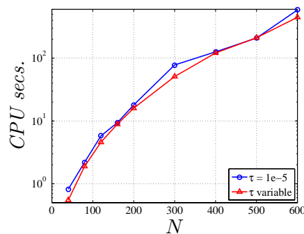
Fig. 15. Comparison of CPU times (right) for the exponential blow-up problem.
